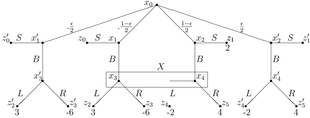
Figure 5: The transformed match nature game
