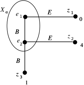
Figure 2: The absentminded driver game.
