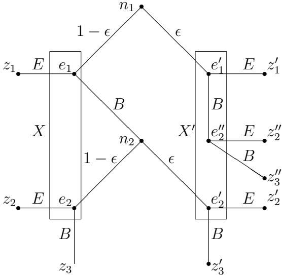
Figure 4: The transformed absentminded-driver game
