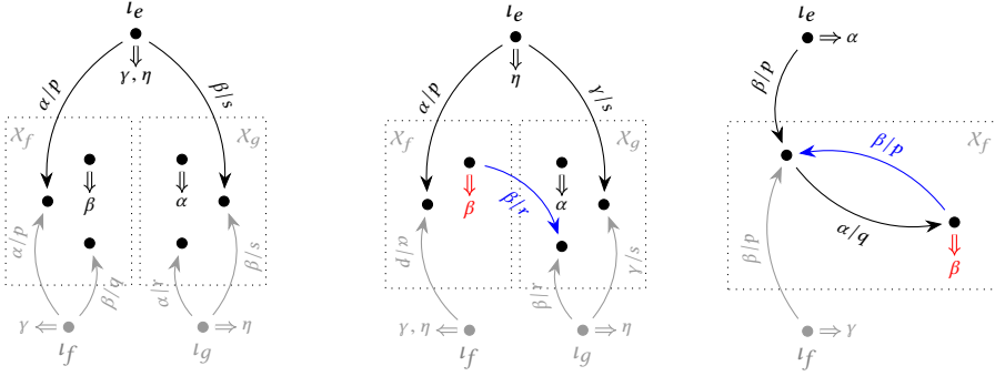
(a) e = f +_b g , with \alpha, \gamma \leq b and \beta, \eta \leq \bar{b} . (b) e = f \cdot g (c) e = f^{(b)} , with \beta, \gamma \leq b and \alpha \leq \bar{b}
