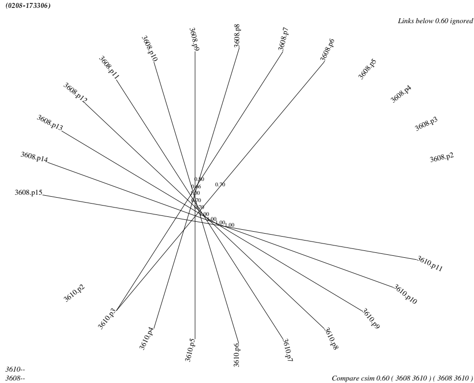
Figure 5: Document-Document Text Relationship Map for Articles 3608 and 3610. A line connects two paragraphs if their similarity is above a predefined threshold.
