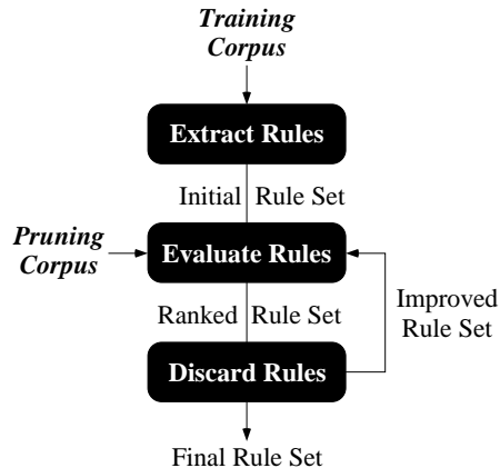
Figure 1: Error-Driven Pruning of Treebank Grammars
