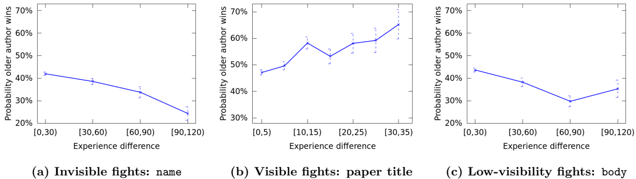
Figure 3: Percentage of fights won by the older author as a function of difference in experience. The larger the experience gap, the more likely the younger author is to win the (invisible) macro name fights (a) and the (low-visibility) macro body fights (c); the opposite trend holds for the (much more visible) title fights (b).
