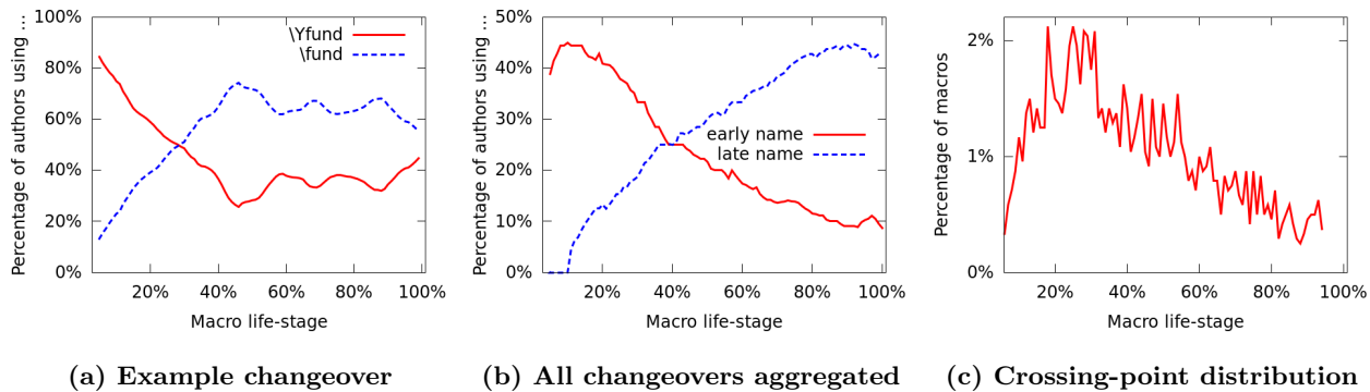
Figure 1: Changeover in conventions. (a) An example changeover: \fund surpasses the once-dominant \Yfund as the preferred name used to invoke Young tableau; y-axis indicates the percentage of users of each name out of all authors using the respective body. (b) Aggregated temporal usage trends of early name ( N_e ) and late name ( N_\ell ) for all macros undergoing changeovers; their crossing point is well before the middle of their lifespan. (c) The distribution of crossing points (percentage out of all macros undergoing changeovers).
